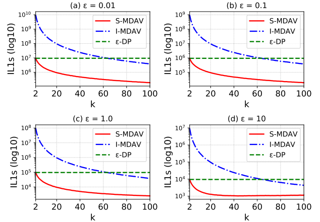
Figure 6: Evolution of ILIs using S-MDAV, I-MDAV and \epsilon -DP for different values of k and \epsilon in EIA.
