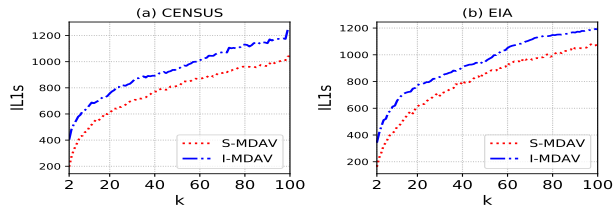
Figure 4: Evolution of ILIs using MDAV and I-MDAV for different values of k : (a) CENSUS and (b) EIA.
