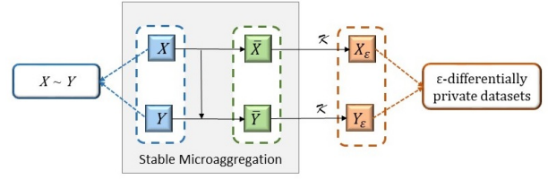
Figure 3: Proposed framework to generate \epsilon -differentially private datasets via stable microaggregation.
