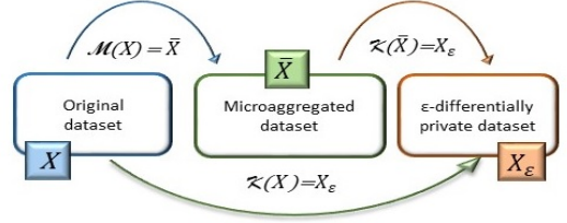
Figure 1: Problem setting.
