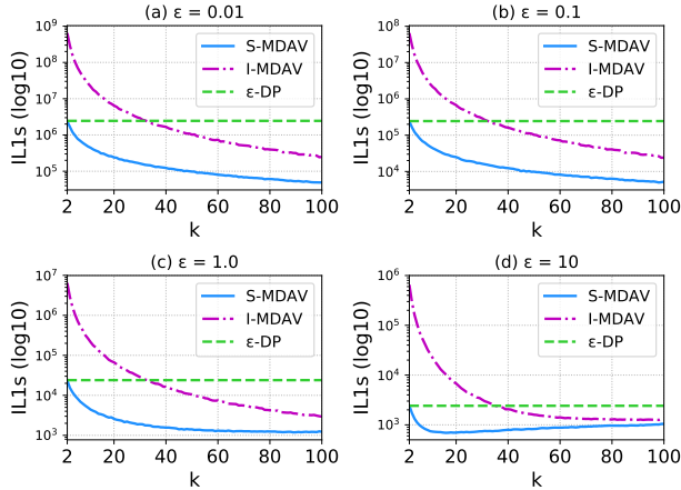
Figure 5: Evolution of ILIs using S-MDAV, I-MDAV and \epsilon -DP for different values of k and \epsilon in CENSUS.
