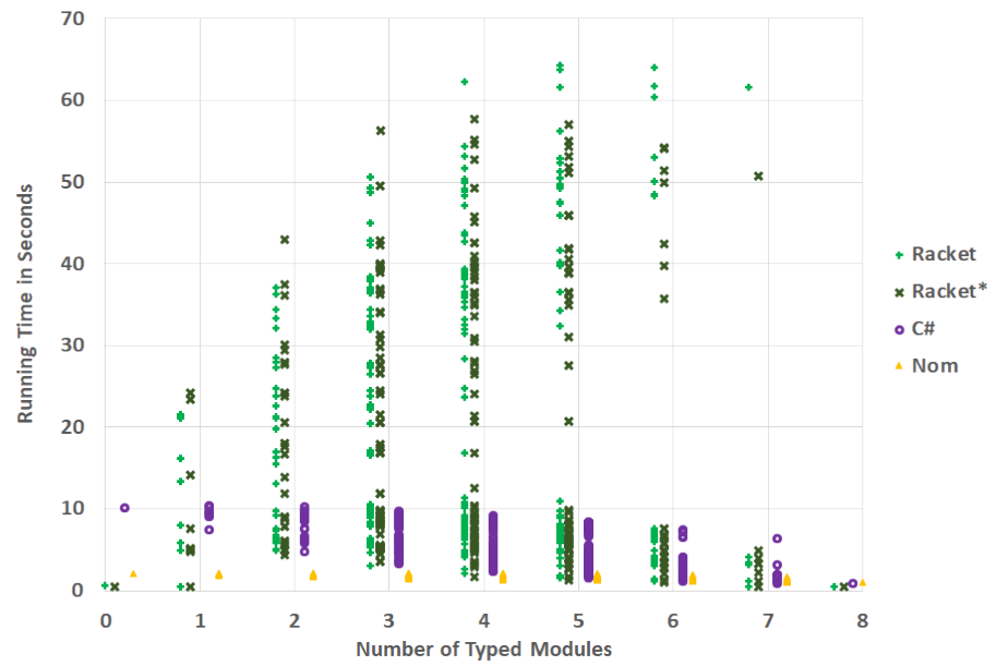
Figure 5.10: Benchmark results for sieve (top) and snake (bottom)
