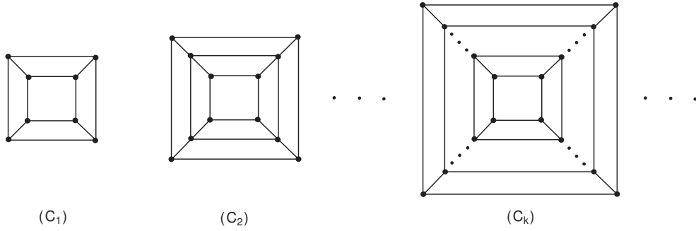
Figure 1: The set S of starting graphs
