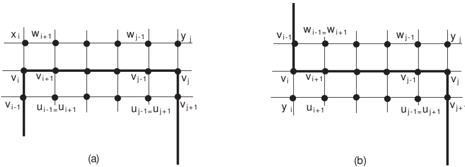
Figure 7: Bent paths in the proof of Theorem 1 (path p is drawn as a thick line)
