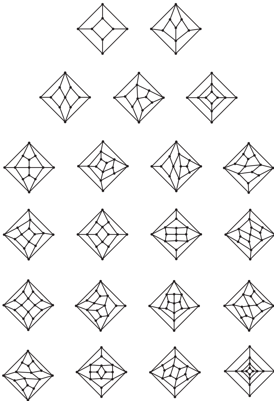
Figure 10: All SPQ(3,4)s with size at most 16.
