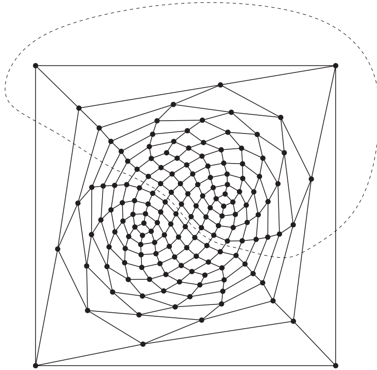
Figure 9: An SPQ(3,4) without any P_1 reductions
