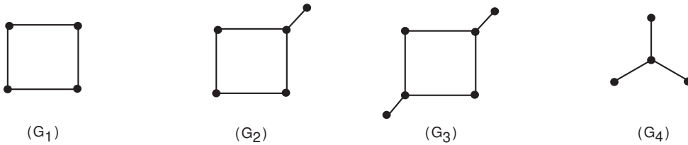
Figure 4: Subgraphs for Lemma 2
