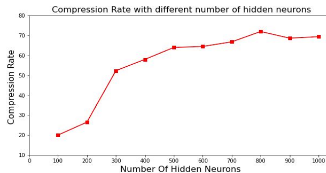
Fig.5 Compression rate with different number of hidden neurons. Compression rate increased as the number of hidden neurons increased.
