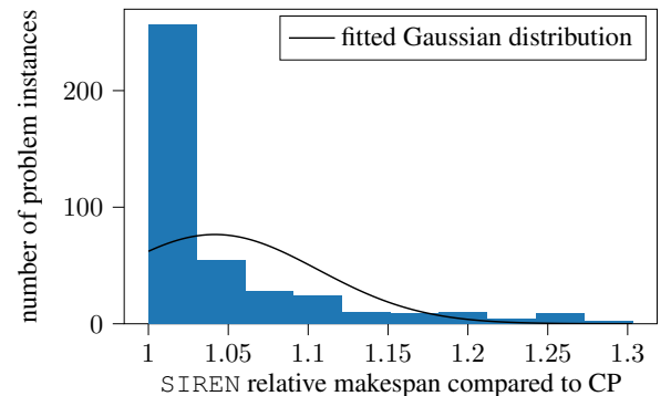
Figure 5: Performance of SIREN relative to the best CP solutions found within a timeout of 15 minutes. On average, SIREN performs 4.2% worse than CP
