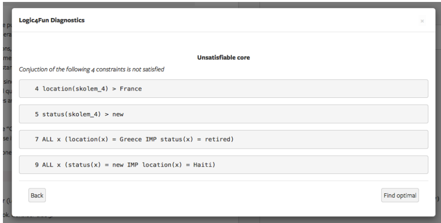
Figure 5: Screenshot of diagnosis tool: unsatisfiable core
