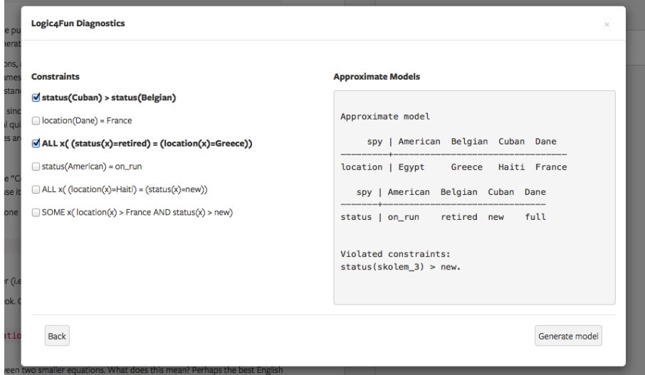
Figure 4: Screenshot of diagnosis tool: approximate model
