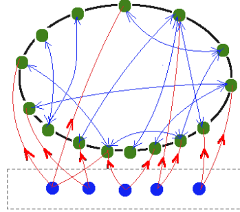
Figure 3. An illustration of a toy-sized map-graph G(V,E) . Green nodes are the 3D point clouds in the map. Blue edges are co-visibility links. The blue nodes on the bottom represent 2D query features which assign initial probabilities to the 3D points based on the query-vector \mathbf{q} computed by Eq.2.
