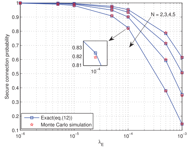
Fig. 1. Monte Carlo simulation results of SCP for colluding eavesdroppers case. The squares represent (12). The stars show the Monte Carlo simulation of (8).
