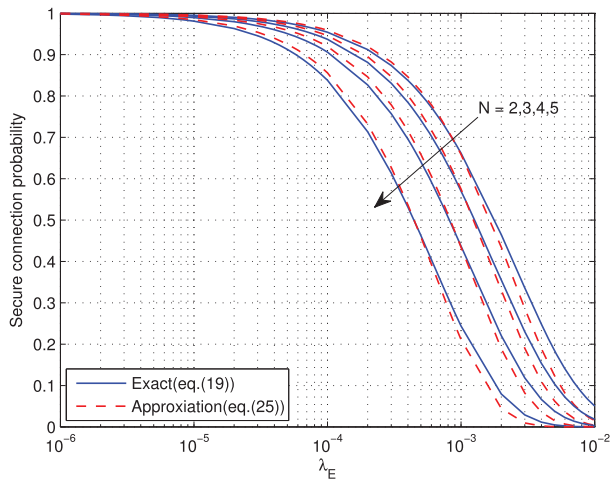
Fig. 4. SCP for non-colluding eavesdroppers case. The solid lines represent (19) and the dashed lines denote SCP approximation (25).
