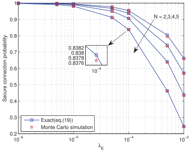
Fig. 3. Monte Carlo simulation results of SCP for non-colluding eavesdroppers case. The squares represent (19). The stars show the Monte Carlo simulation of (14).
