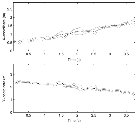
Fig. 8. Tracking results for one run of algorithm SBF-PL using real audio data, showing the true source trajectory (dotted line) and the estimated path resulting from the particle filter (solid line). Grey lines represent \pm one standard deviation of the particle set from its weighted mean (estimated source position \hat{\ell}_s ).
