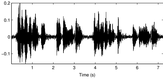
Fig. 2. Typical microphone signal simulated with the image method for RT_{60} = 150\text{ms} .
