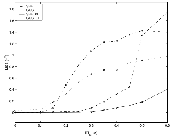
Fig. 4. Average error for two classical and two PF-based source localization methods, plotted vs. reverberation time. The audio data was simulated with the image method for small room acoustics.
