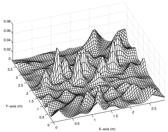
Fig. 7. Beamformer output power function used as pseudo-likelihood in algorithm SBF-PL, for one signal frame.
