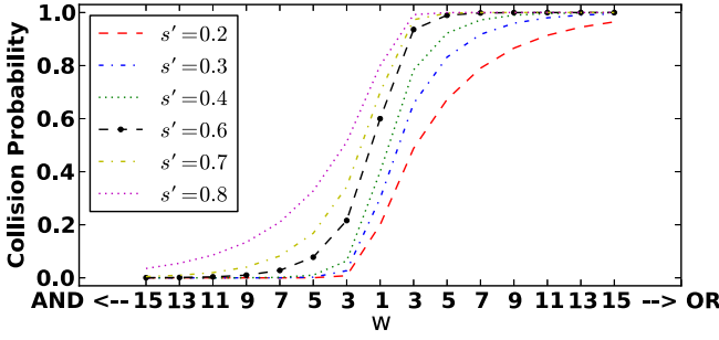
Fig. 5. The collision probability of a w -way semantic hash function under different semantic similarities s' , where w = 1, 2, \dots, 15 and \mu \in \{\wedge, \vee\} .
