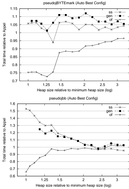
Figure 10: Total execution time, for best configuration (continued).
