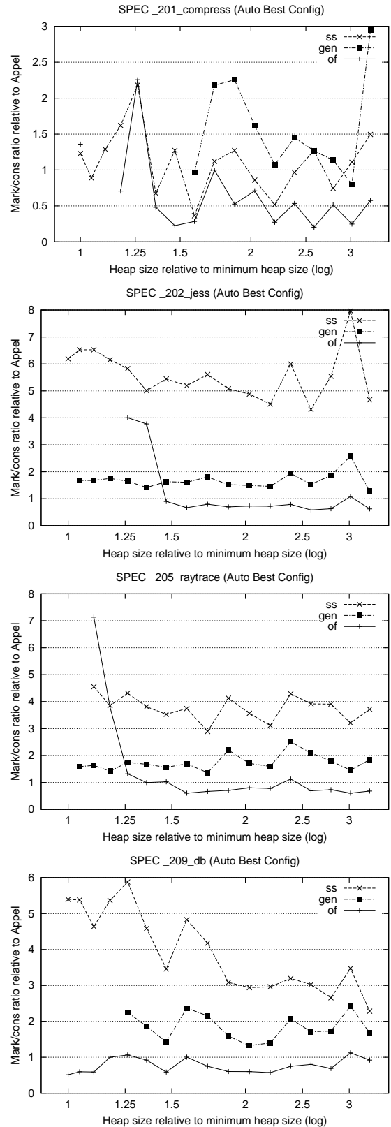
Figure 11: Mark/cons ratio, for best configuration.
