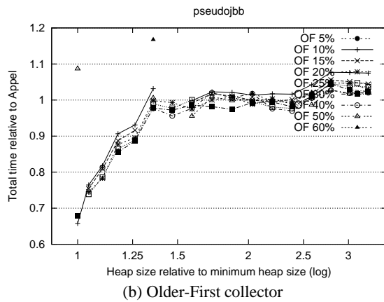
Figure 6: Total execution time: pseudojbb .
