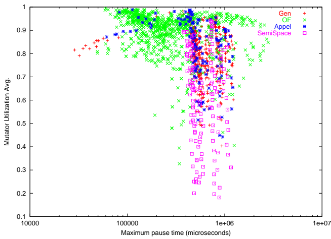
Figure 14: Mutator utilization vs. maximum pause time, all program runs.
