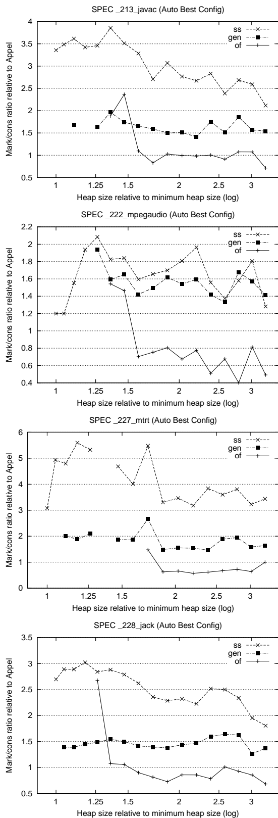
Figure 12: Mark/cons ratio, for best configuration (continued).
