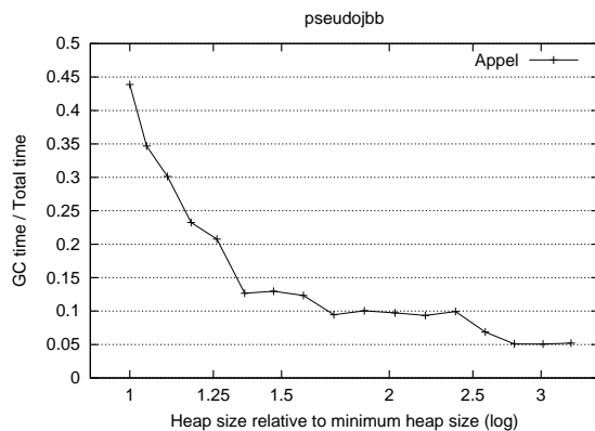
Figure 7: GC time as fraction of total execution time (Appel collector): pseudojbb .
