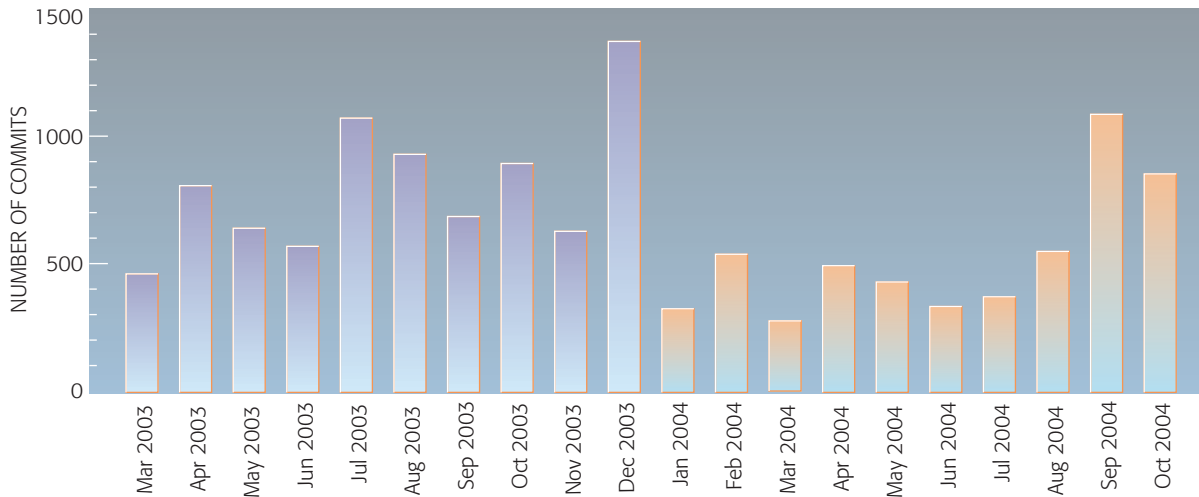
Figure 5 CVS commits
