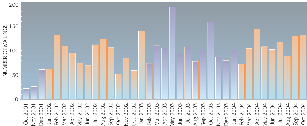
Figure 3 Mailing-list traffic
