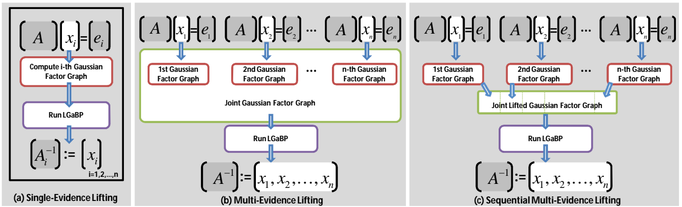
Figure 2: Inverting a matrix A using multi-evidence lifting. (a) Single-evidence lifting runs LGaBP solving Ax_i = e_i for each i = 1, 2, \dots, n separately; e_i denotes the i th basis vector; thus LGaBP computes each column vector of A^{-1} separately. (b) Multi-evidence lifting runs LGaBP on the joint graphical model of Ax_i = e_i for i = 1, 2, \dots, n ; thus LGaBP computes A^{-1} for all e_i at once. (c) Sequential multi-evidence lifting directly builds the lifted joint graphical model in a sequential fashion, avoiding cubic space complexity
