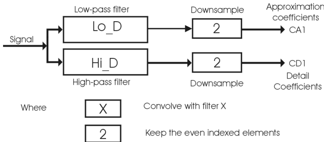
Fig. 2. Mallat wavelet decomposition.
