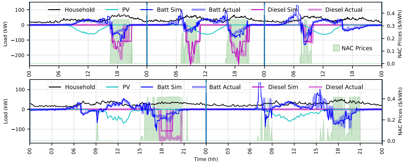
Fig. 6. Battery and diesel response for five days (June 9–11 top, July 20–21 bottom) comparing the actual and simulated values.
