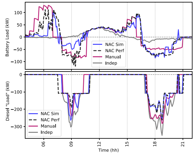
Fig. 8. Aggregate battery (top) and diesel (bottom) power compared for June 10.
