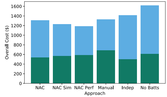
Fig. 7. Diesel (upper segment) and participant (lower segment) costs for different approaches over the 5.5 days for detailed analysis.
