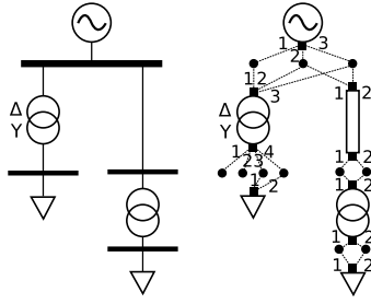
Fig. 3. Left: single line diagram. Right: our explicit representation with nodes (solid circles), elements, terminals (solid squares) and ordered connections for each terminal (numbered dashed lines).
