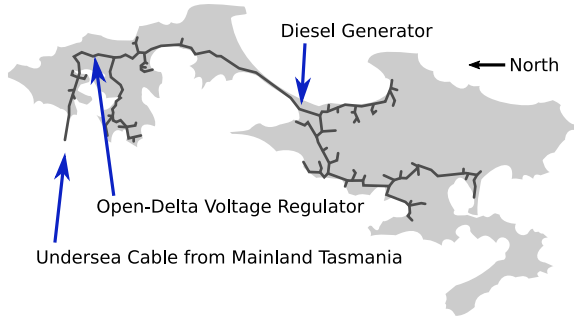
Fig. 1. Bruny Island southern MV feeder.
