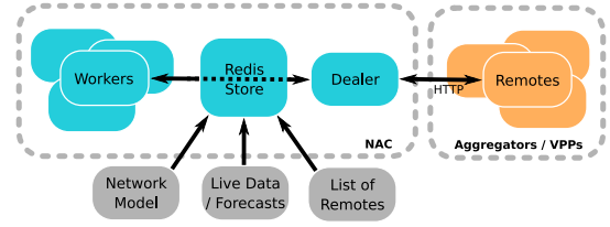
Fig. 5. Structure of the NAC implementation and interaction.
