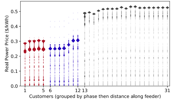
Fig. 9. Histogram of real power LMPs for each customer.
