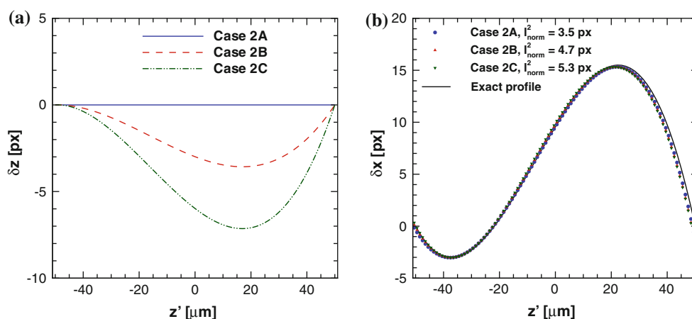
Fig. 9 The effects of out-of-plane velocity component to the velocity measurement accuracy. a Increasing out-of-plane velocities where case 2A has zero magnitude and case 2B has half of the magnitude as compared with that of case 2C. The out-of-plane displacement is
