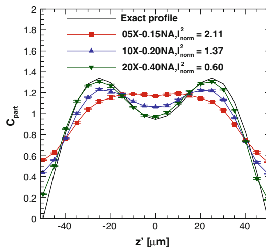
Fig. 6 Concentration measurements obtained from synthetic scanning PIV images using image filtering and particle counting. Solid curves without symbols represent the exact profiles. Symbols with error bars represent the measurement points. Here z' = z z_0 H/2 . The l_{\text{norm}}^2 values represent the total measurement errors across the measurement volume. The measured concentration versus exact concentration follows Eq. 7. Error in concentration measurement decreases as lens numerical aperture increases
