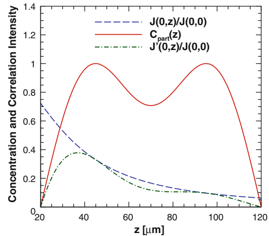
Fig. 4 Effect of particle concentration on the mean intensity of the auto-correlation peak within a channel of 100 \mu\text{m} depth with the focal plane located at z = 0 . For constant concentration, the correlation intensity J(0,z) is as shown by the dash-dash curve . However, with a varying particle concentration C_{\text{part}}(z) ( solid curve ), the effective correlation intensity J'(0,z) shown as dashed-dot is equal to C_{\text{part}}(z) \times J(0,z)
