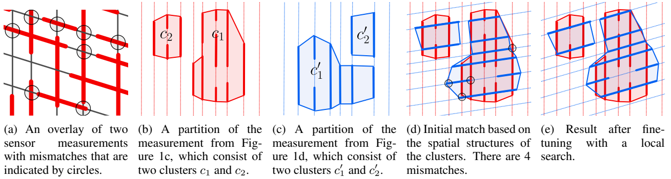
Figure 2: Integration of sensor measurements based on Algorithm 1.
