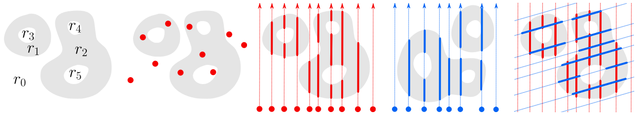
(a) A complex region consisting of positive components r_1, r_2 and negative components r_0, r_3, r_4, r_5 .
