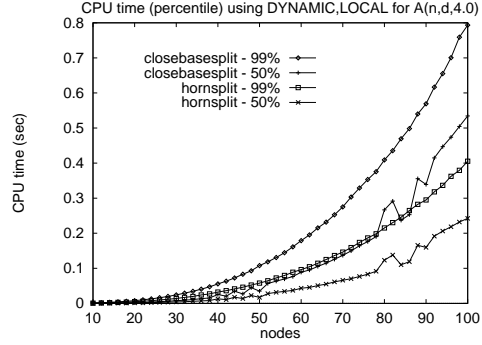
Figure 7. Percentile 50% and 99% CPU time of \hat{H}_8 and \hat{B} for solving A(n, d, 4.0) ( d = 8.0 - 10.0 , 2,500 instances/data point)
