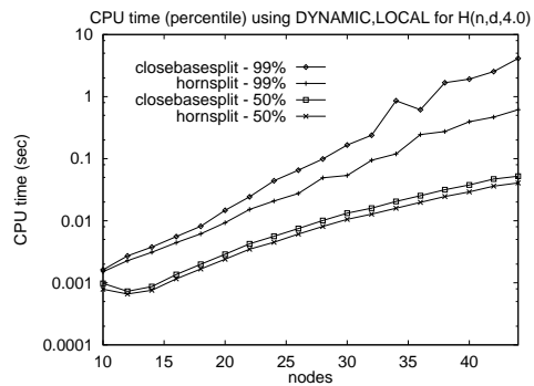
Figure 8. Percentile 50% and 99% CPU time of \hat{H}_8 and \hat{B} for solving H(n, d, 4.0) ( d = 10.0 - 15.0 , 5,500 instances/data point)
