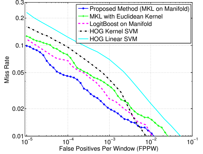
Figure 1: Pedestrian detection. Detection-Error tradeoff curves for the proposed manifold MKL approach and state-of-the-art methods on the INRIA dataset. The curves for the baselines were reproduced from [20].
