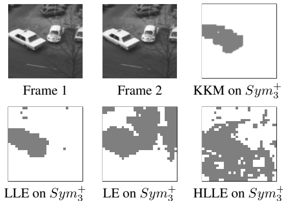
Figure 3: 2D motion segmentation. Comparison of the segmentations obtained with kernel k -means with our Riemannian kernel (KKM), LLE, LE and HLLE on Sym_3^+ . The baseline results were reproduced from [8].
