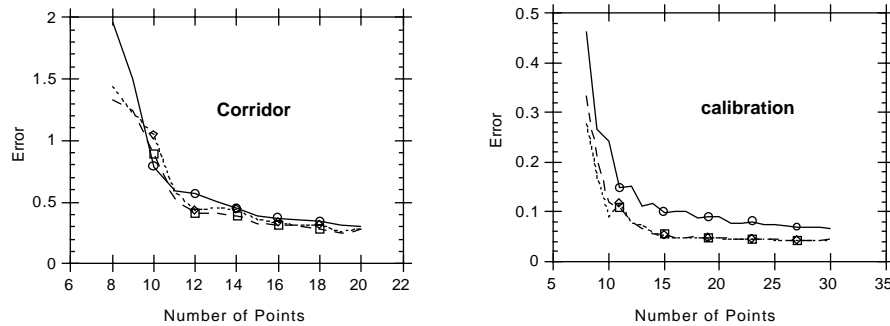
Normalized 8-point, geometric and algebraic error.
