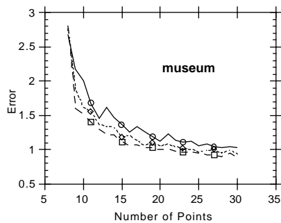
Normalized 8-point, geometric and algebraic error.
