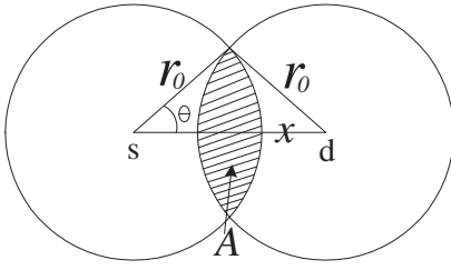
Fig. 1. An illustration of two-hop neighbors. Sensors s and d are two random sensors separated by a distance x ( r_0 < x \leq 2r_0 ).
