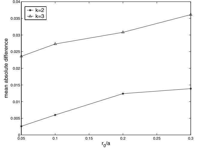
Fig. 4. MAD between the analytical results and the corresponding simulation results for different values of r_0/a ; \pi r_0^2 \rho is kept constant at 15.7080. When r_0/a increases, a larger percentage of sensors are located near the boundary and the impact of the boundary effect is more pronounced. Thus the discrepancy between the analytical and the simulation results increases.
