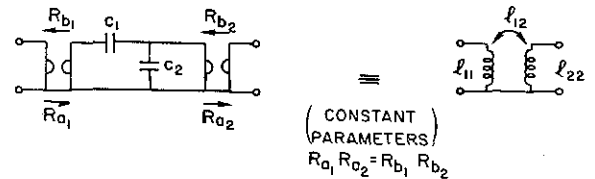
Fig. 2. Coupled coil simulation.
