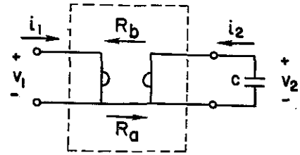
Fig. 1. Variable inductor simulation.
