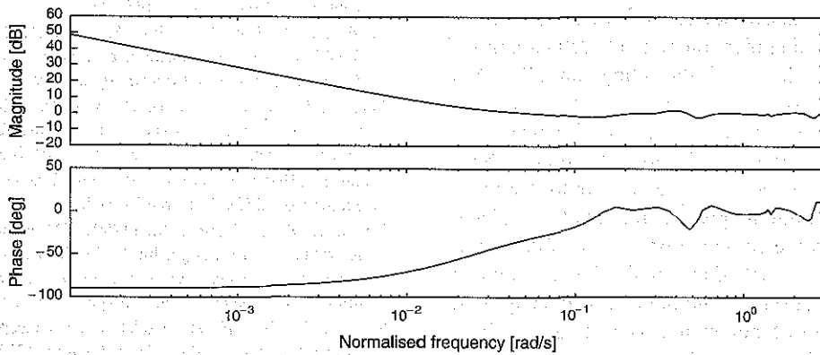
Fig. 5. Coprime-factor approach using r_2(t) : Bode diagram of \hat{T}_{22} + \hat{T}_{12}K .
