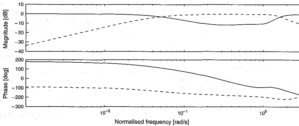
Fig. 6. Bode diagrams of the normalised coprime factors of K : U (—) and V (---).
