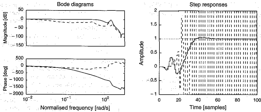
Fig. 4. Control design via coprime-factor identification using r_1(t) : Bode diagrams (left) and step responses (right) of \bar{F}\hat{G}/(1 + \bar{K}\hat{G}) (—) and \bar{F}G_0/(1 + \bar{K}G_0) (---).
