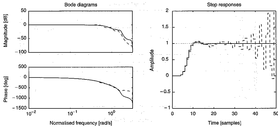
Fig. 3. Control design via indirect identification using T_{12} : Bode diagrams (left) and step responses (right) of \bar{F}\hat{G}/(1+\bar{K}\hat{G}) (—) and \bar{F}G_0/(1+\bar{K}G_0) (---).
