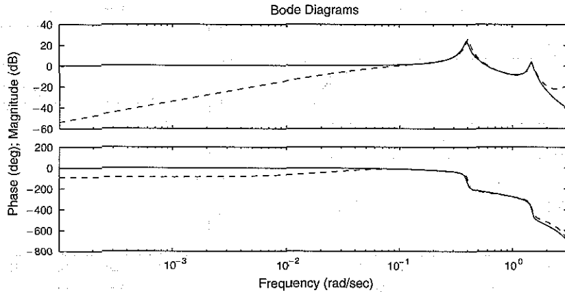
Fig. 2. Indirect identification using T_{12} : Bode diagrams of G_0 (—) and \hat{G} (---).
