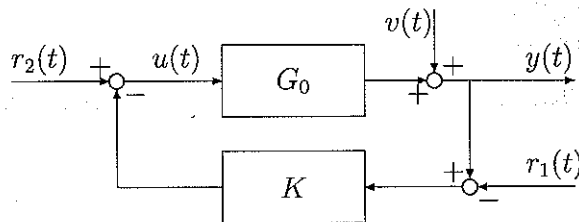
Fig. 1. Closed-loop system.
