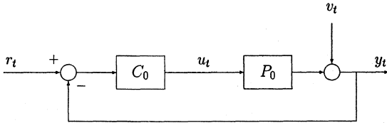
Fig. 1. One degree of freedom control loop.
