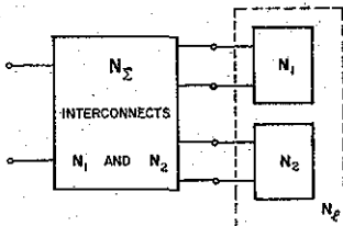
Fig. 2.—General Interconnection of Two Reciprocal Networks.
