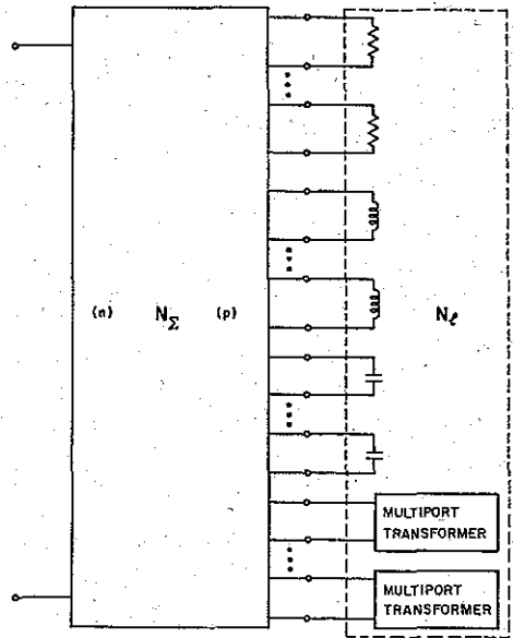
Fig. 1.—Cascade Loading Representation of N .
