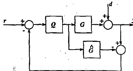
Figure 2. IMC structure
