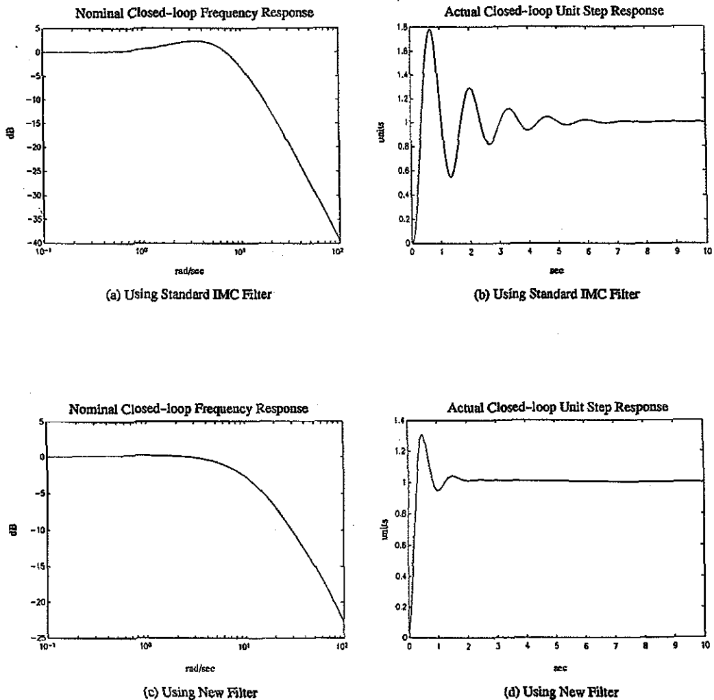
Figure 11. Frequency and step responses when bandwidth is 10 rad/s and \gamma is 0.3
