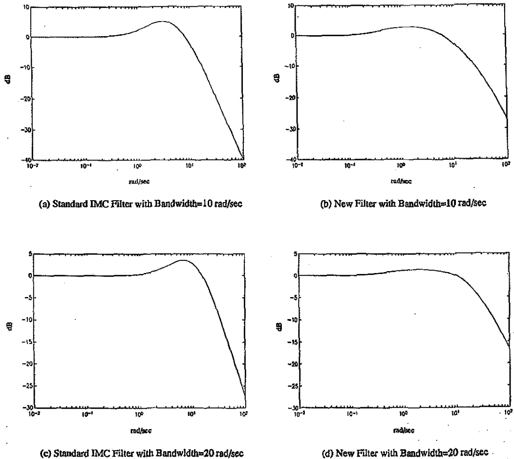
Figure 5. Frequency responses of standard IMC filter and new filter with \gamma = 0.5
