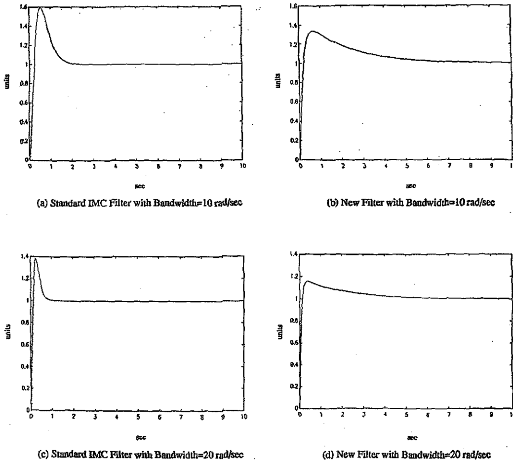
Figure 6. Step responses of standard IMC filter and new filter with \gamma = 0.5
