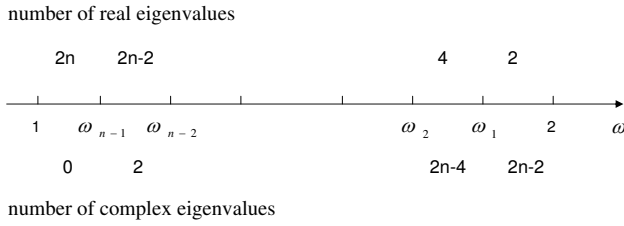
Fig. 1. Distribution of \bar{B} 's real and complex eigenvalues
