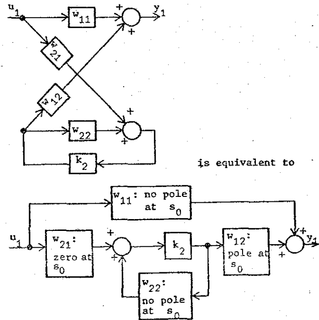
Figure 1: Illustration of fixed mode leading to uncontrollability.
