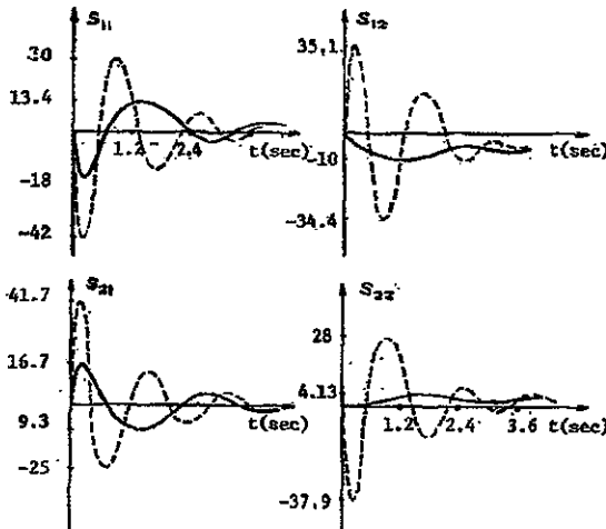
Figure 2: Plant Inputs ( s_{ij} : Plant Input i for step on reference input j )
