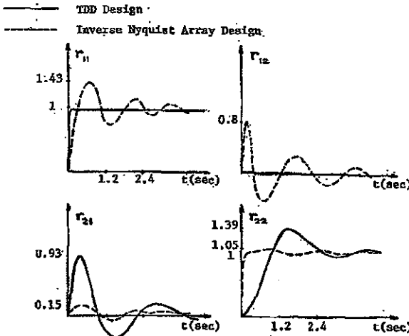
Figure 1: Output Step Responses. ( r_{ij} : Plant Output i for step on reference input j )
