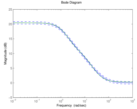
Fig. 3. The model G and the second-order approximation G_a obtained in Example 1. The uniform bounds are plotted with dashed lines. Here \gamma = 0.1 , which gives an error bound of 0.38 dB.
