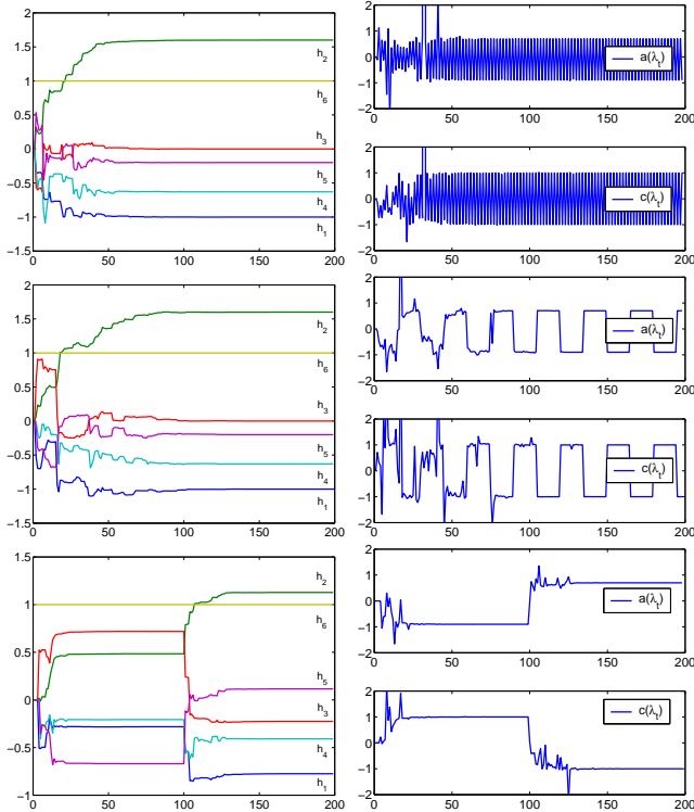
Fig. 1. Evolution of \hat{h}_t (left), \hat{a}(\lambda_t) and \hat{c}(\lambda_t) (right) for \Pi_2 \hat{h}_0 = 0 , \sigma = 0 and \lambda_t of period of 2 (top), 30 (middle) and 200 seconds (bottom).
