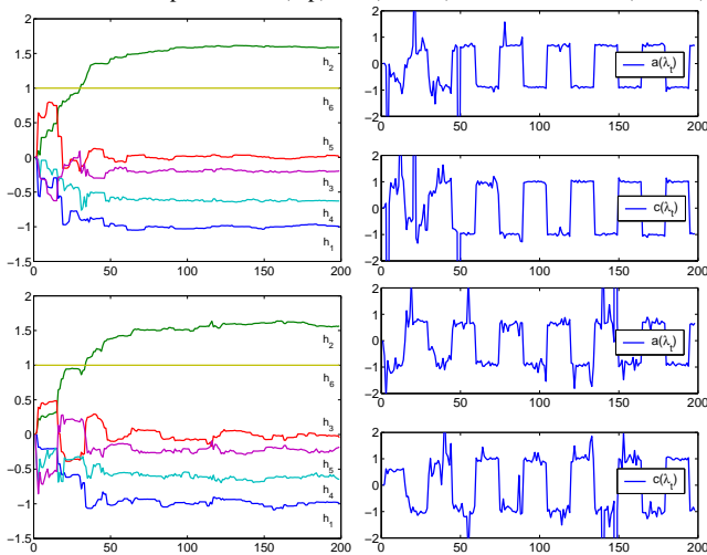
Fig. 2. Evolution of \hat{h}_t (left), \hat{a}(\lambda_t) and \hat{c}(\lambda_t) (right) for \Pi_2 \hat{h}_0 = 0 , \lambda_t of period 30 seconds, \sigma = 0.02 (top) and \sigma = 0.05 (bottom).
