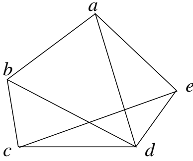
Fig. 2. A globally rigid formation in the plane.
