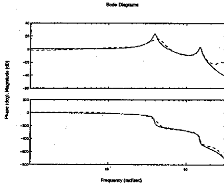
Fig. 3. Joint i/o approach: P_0 (—), \hat{P} (---)
