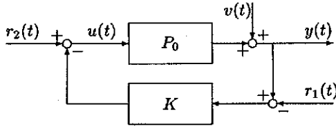
Fig. 1. Closed-loop system
