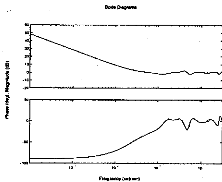
Fig. 4. Joint i/o approach: \hat{T}_{22} + \hat{T}_{12}K
