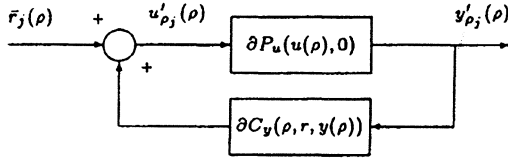
Figure 2.2: Generation of u'_{\rho_j}(\rho) and y'_{\rho_j}(\rho)
