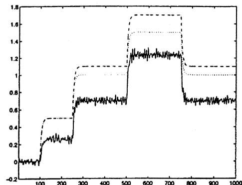
Figure 3.1: Reference signal ( \cdots ), desired closed loop response ( --- ) and achieved closed loop response with the initial controller ( — ).
