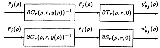
Figure 2.3: Generation of u'_{\rho_j}(\rho) and y'_{\rho_j}(\rho)
