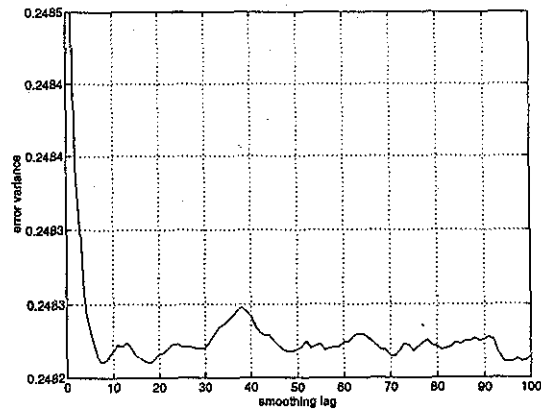
Figure 2: Variation of smoothing error with \Delta : A fixed, C_2 ; filter error: 0.2487
