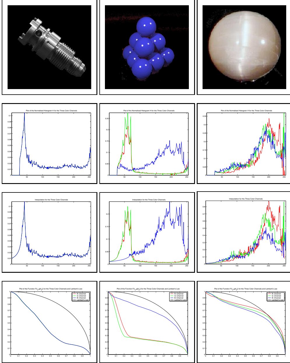
Fig. 6. Input images and plots of the variables computed through the radiance function approximation process.
