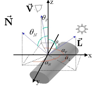
Fig. 1. Geometry of the reflection process
