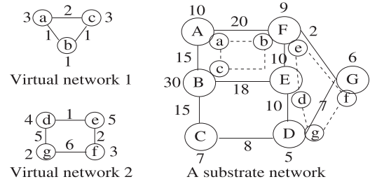
Fig. 2. Virtual network embedding.
