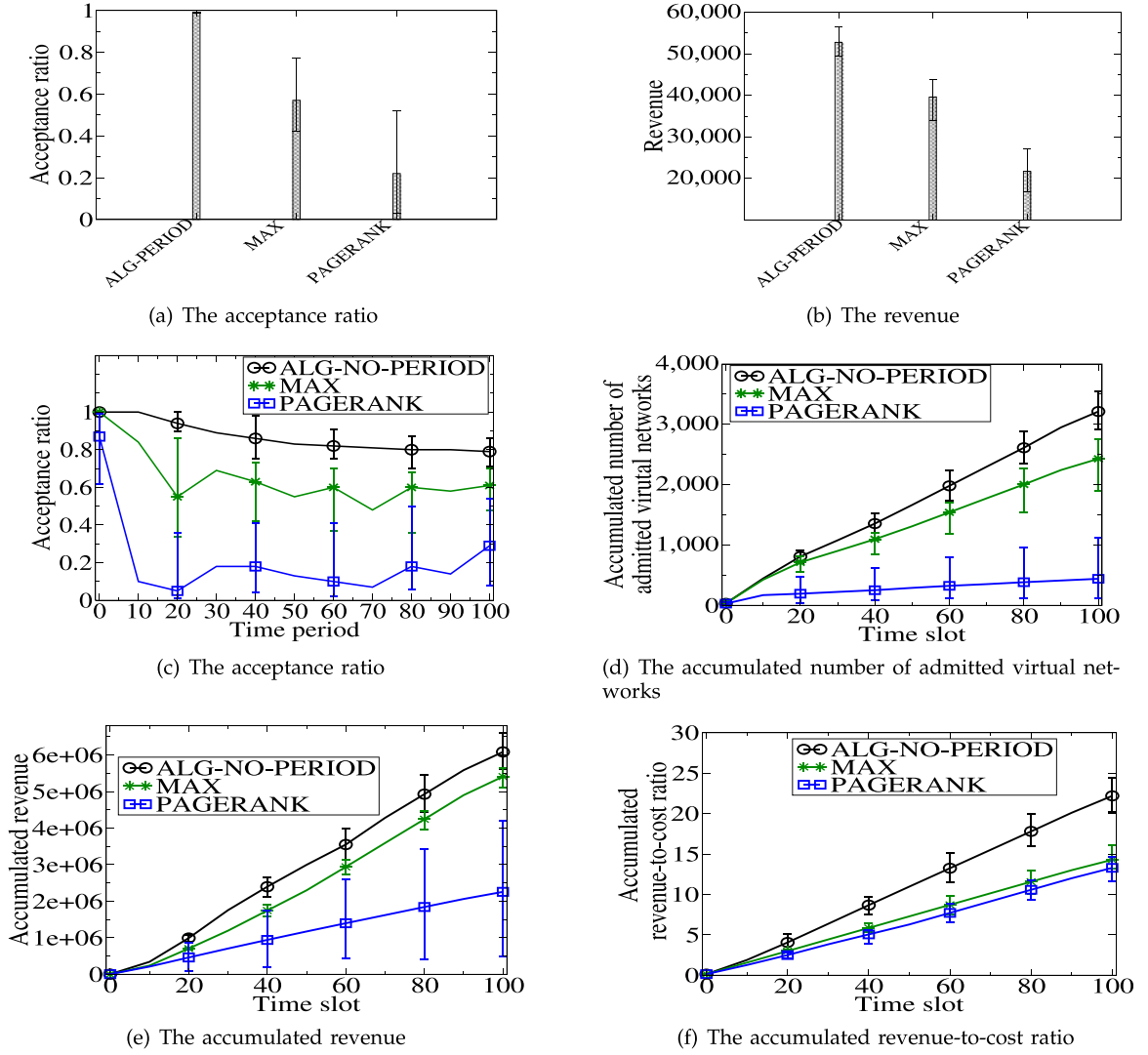
Fig. 4. The performance of different algorithms under Weekday-weekend resource demand patterns.
