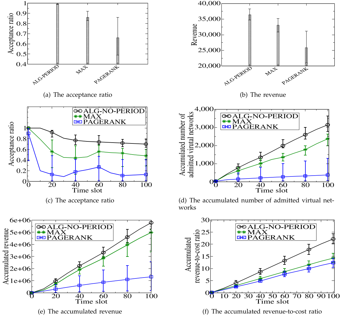
Fig. 3. The performance of different algorithms under Random resource demand patterns of virtual networks.
