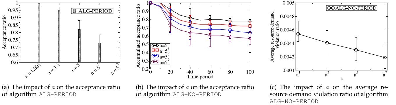
Fig. 7. The impact of a on the performance of different algorithms.
