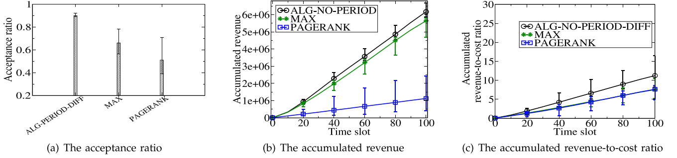
Fig. 5. The performance of different algorithms with different resource demand periods and under Random resource demand patterns of virtual networks.
