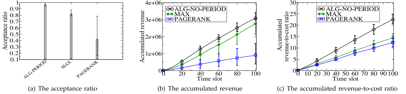
Fig. 6. The performance of different algorithms using GÉANT topology under Random resource demand patterns of virtual networks.
