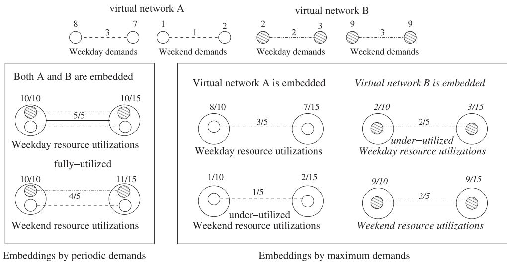
Fig. 1. A motivated example of resource sharing among virtual networks with periodic resource demands.
