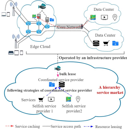
Fig. 1. An example of the two-tiered cloud network.
