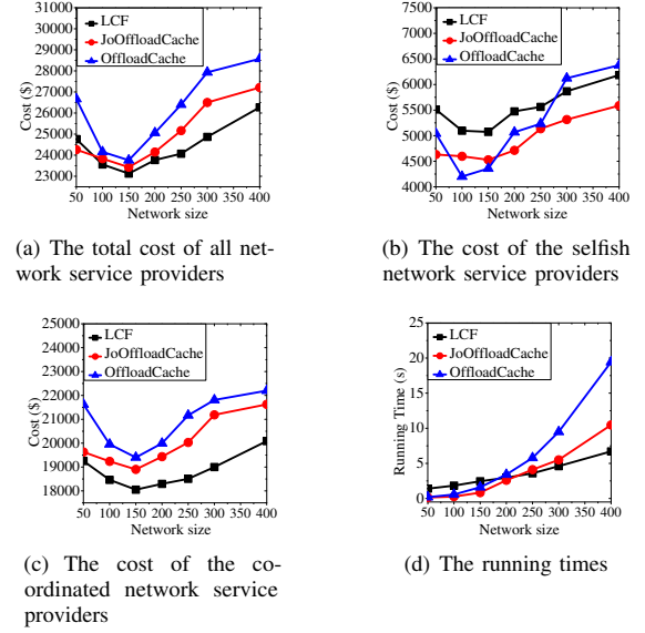
Fig. 2. Algorithm performance in GT-ITM generated networks with sizes varied from 50 to 400.
