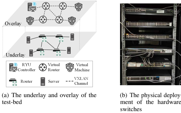
Fig. 4. A test-bed with both hardware switches and virtual resources.
