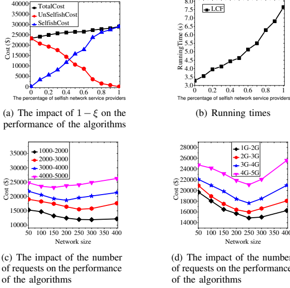
Fig. 6. Results of the impact of the ratio of the number of coordinated network service providers and selfish ones in the test-bed.
