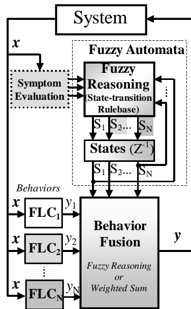
Fig. 1. The proposed behaviour-based control structure.
