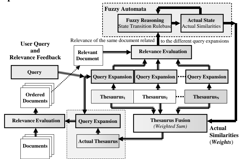
Fig. 5: Structure of the proposed adaptive thesaurus generation.
