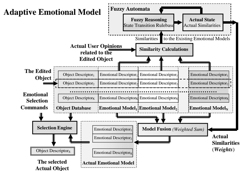
Fig. 4: Structure of the proposed adaptive emotional model generation.
