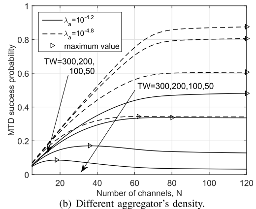
Fig. 6. Number of channels, N , versus the MTD success probability with (a) different path-loss exponent and (b) different aggregator's density.
