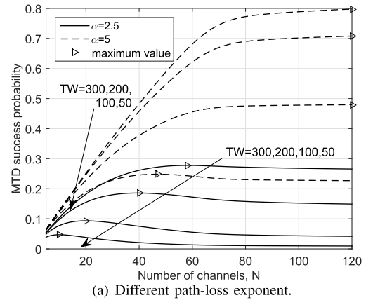
(a) Different path-loss exponent.
