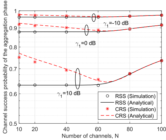
Fig. 2. Channel success probability of the aggregation phase, \bar{p}_{suc1}^r , versus the number of channels, N , with \bar{m} = 70 and different SIR threshold for both of the RRS and CRS.
