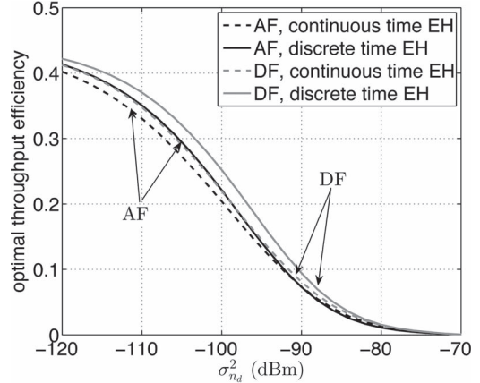
Fig. 8. Optimal throughput efficiency versus destination noise variance, \sigma_{n_d}^2 , for TS-based protocols for EH and IT in AF and DF relaying with continuous time and discrete time EH.
