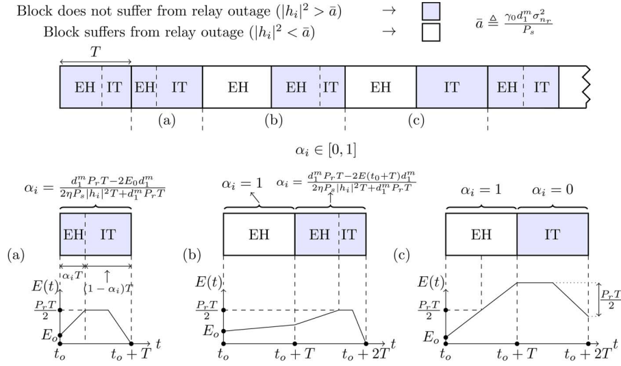
Fig. 3. Illustration of TS-based protocol for EH and IT in DF relaying, with continuous time EH, \alpha_i \in [0, 1] for three different EH-IT block (a) single EH-IT block (b) n = 1 EH block due to relay outage followed by an EH-IT block and (c) n = 1 EH block due to relay outage followed by an IT block. n is the random number of successive EH blocks due to relay outage, occurring irrespective of accumulated energy, in continuous time EH (DF only).
