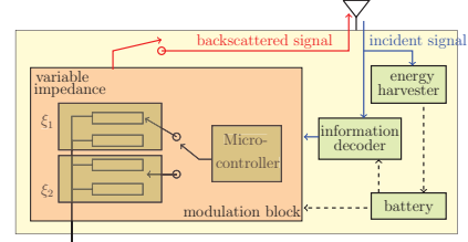
Fig. 1. Illustration of the structure of BN.
