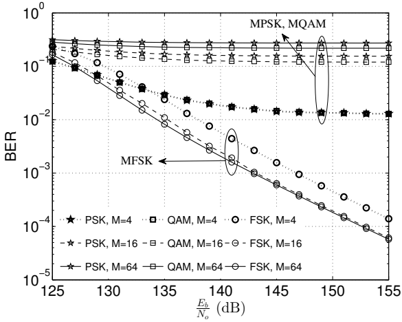
Fig. 3. BER versus \frac{E_b}{N_o} at the transmitter (reflects to \frac{E_b}{N_o} = \{1, 6, \dots, 31\} dB at the receiver) with hardware distortion noise variance \sigma_{nl}^2 = 0.2 .
