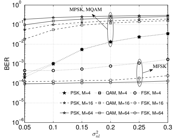
Fig. 4. BER versus hardware distortion noise variance \sigma_{nl}^2 at \frac{E_b}{N_o} = 150 dB at the transmitter (reflects to \frac{E_b}{N_o} = 26 dB at the receiver).
