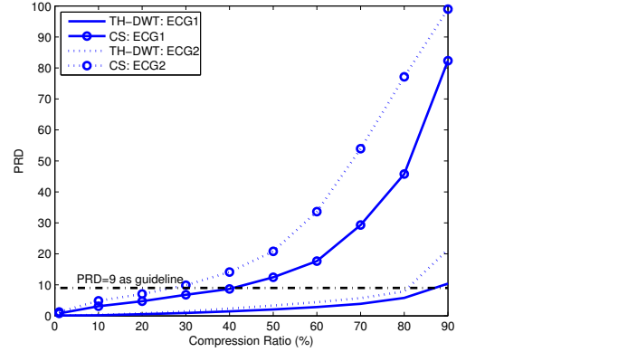
Fig. 2: ECG recovery performance versus compression ratio.
