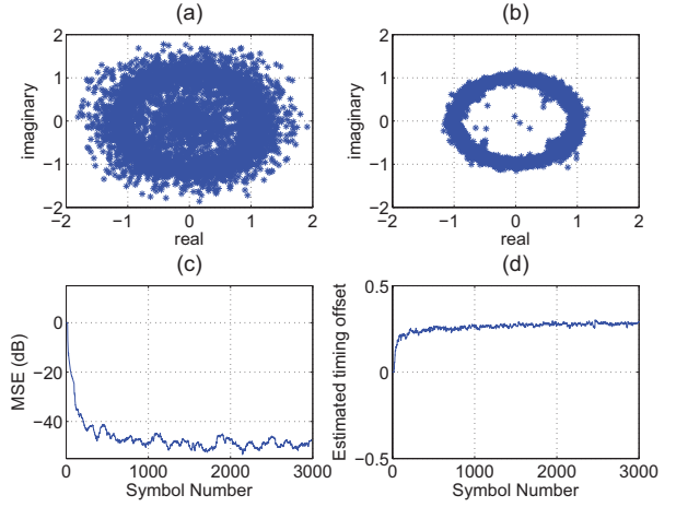
Fig. 3. Results for FSE with multipath channel, fractional timing phase offset ( \tau ) = -0.3, frequency offset ( \Delta f/F_s ) = 10^{-2} , SNR = 20 dB, DQPSK and equalizer length N_f = 7 . (a) Channel output constellation. (b) Equalized output constellation. (c) MSE between equalizer output and transmitted symbols. (d) Timing offset recovery.
