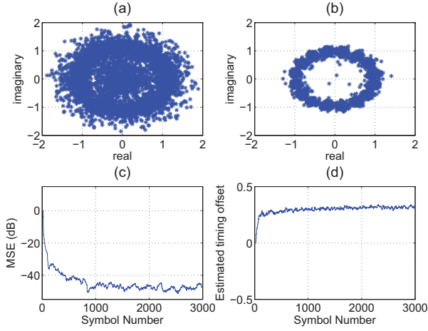
Fig. 2. Results for TSE with multipath channel, fractional timing phase offset ( \tau ) = -0.3, frequency offset ( \Delta f/F_s ) = 10^{-2} , SNR = 20 dB, DQPSK and equalizer length N = 7 . (a) Channel output constellation. (b) Equalized output constellation. (c) MSE between equalizer output and transmitted symbols. (d) Timing offset recovery.
