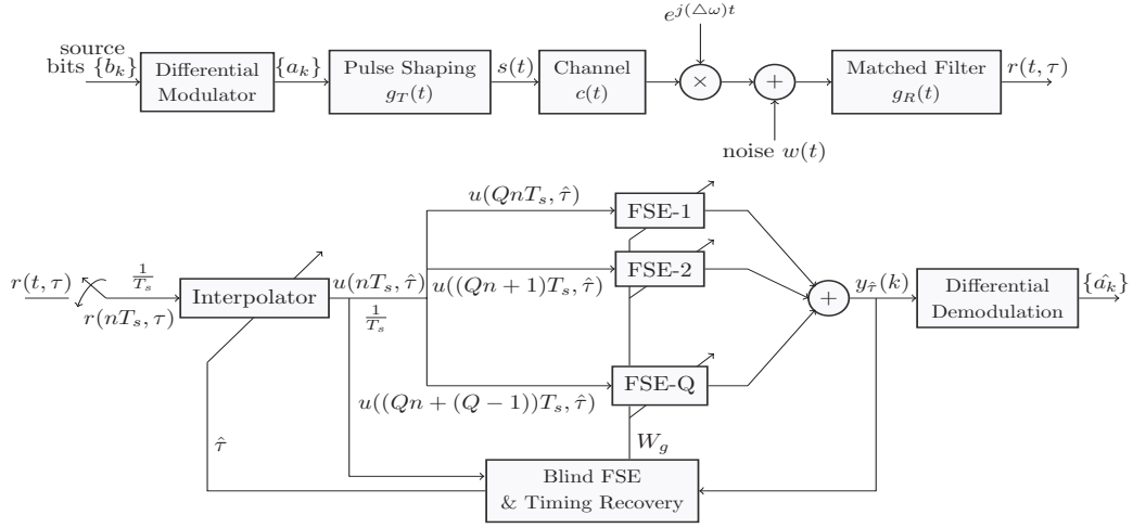
Fig. 1. Baseband Communication System for Blind Synchronization and Fractionally Spaced Equalization.
