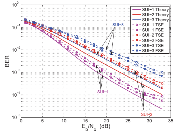
Fig. 5. BER versus E_b/N_o (dB) for SUI fading channels with Sampling Time T_s = 0.1\mu s , FSE length N_f = 10 , TSE length N = 10 and Differential QPSK modulation.
