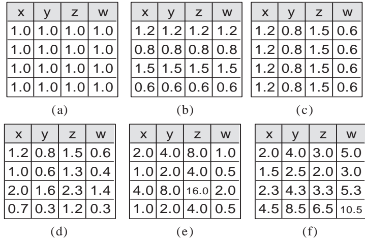
Fig. 4. The six different types of bi-clusters: (a) constant block bi-cluster; (b) constant row bi-cluster; (c) constant column bi-cluster; (d) additive coherent bi-cluster; (e) multiplicative coherent bi-cluster; (f) row-wise linear coherent bi-cluster
