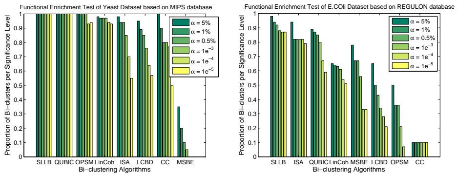
Fig. 15. Portions of discovered bi-clusters by the eight algorithms on the two real datasets that are significantly enriched in the MIPS pathway experimentally verified REGULONS, respectively, using six different P -value cutoffs.
