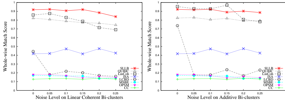
Fig. 7. The overall match scores of the eight algorithms for recovering linear coherent and additive bi-clusters, at six different noise levels.
