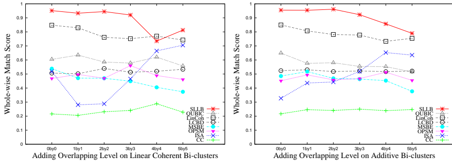
Fig. 9. The whole match scores of the eight algorithms for recovering the overlapping linear coherent and additive bi-clusters, under the adding overlap model.
