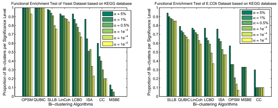
Fig. 14. Portions of discovered bi-clusters by the eight algorithms on the two real datasets that are significantly enriched in the KEGG pathway, using six different P -value cutoffs.
