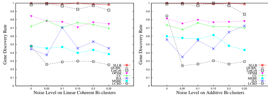
Fig. 8. The gene discovery rates of the eight algorithms for recovering linear coherent and additive bi-clusters, at six different noise levels.
