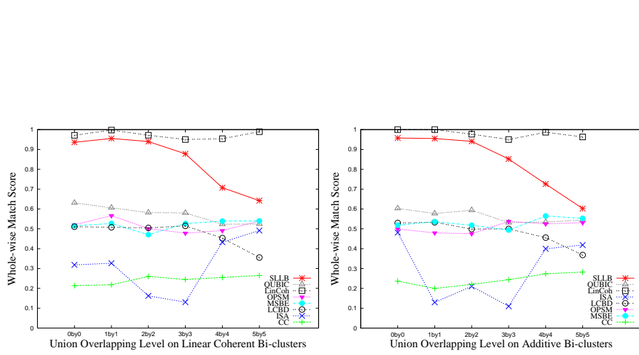
Fig. 12. The whole match scores of the eight algorithms for recovering the overlapping linear coherent and additive bi-clusters, under the union overlap model.
