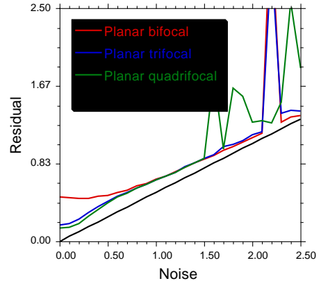
Figure 2: Comparison of the three planar methods (bifocal, trifocal and quadrifocal) applied to the room sequence (without bundle adjustment). The theoretical minimum is shown in black. All three methods perform well, within about 10% of the theoretical minimum. The trifocal and quadrifocal methods perform slightly better than the bifocal method at low noise levels. The deviations at high noise levels are due to occasional failure of the algorithm, but these noise levels are beyond practical noise limits.
