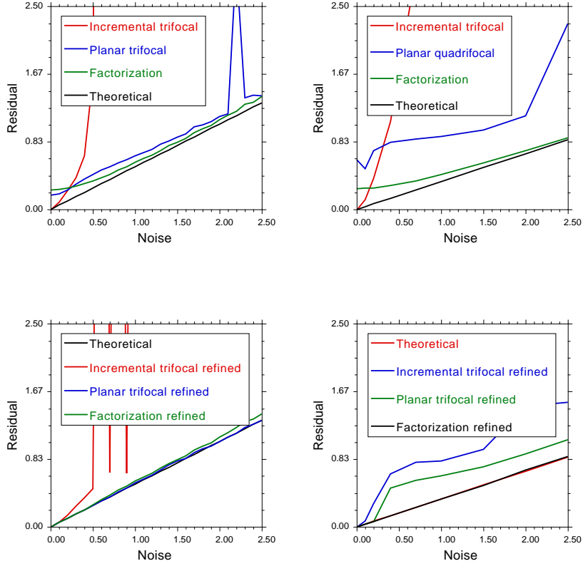
Figure 3: Comparison of the trifocal-planar method with the factorization and incremental-trifocal methods, as well as the theoretical minimum ground-truth error. Above are the results for the method alone, below the results after bundle adjustment. The graphs on the left correspond to the room sequence and the ones on the right to the boat sequence. Note that both the planar and factorization methods are better than the incremental method for both sequences. The factorization method performs slightly better than the planar method, but after bundle adjustment both are nearly optimal at low noise, and at all noise levels in the room sequence.
