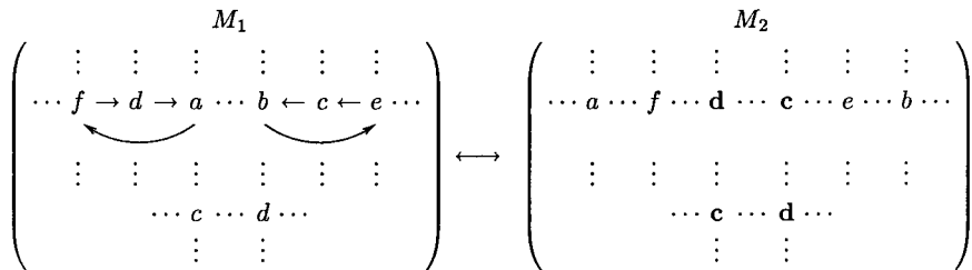
FIG. 1. In the left hand matrix ( M_1 ) two triples of entries in the same row are cycled, to produce a new intercalate in the right hand matrix ( M_2 ). Naturally, the switching process can be reversed in order to destroy the intercalate in M_2 .
