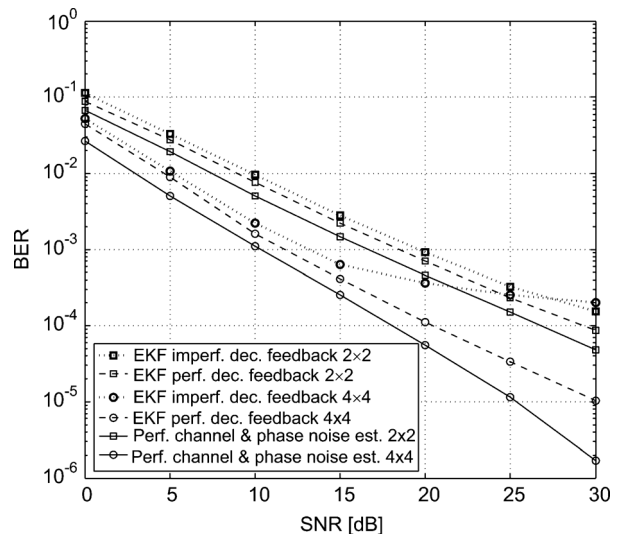
Fig. 11. Perfect and Imperfect decision feedback BER of a MIMO system for different N_t and N_r values, (BPSK modulation, \sigma_{\Delta}^2 = 10^{-4} \text{ rad}^2 , and L_p = 10 ).
