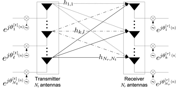
Fig. 1. System model for a point-to-point MIMO systems.
