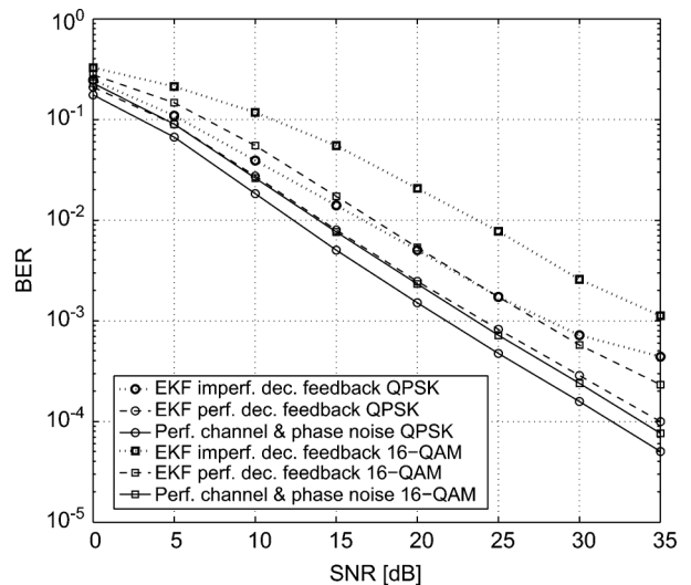
Fig. 10. BER of a 2 \times 2 MIMO system for QPSK and 16-QAM modulations ( L_p = 10 and \sigma_{\Delta}^2 = 10^{-4} \text{ rad}^2 ).
